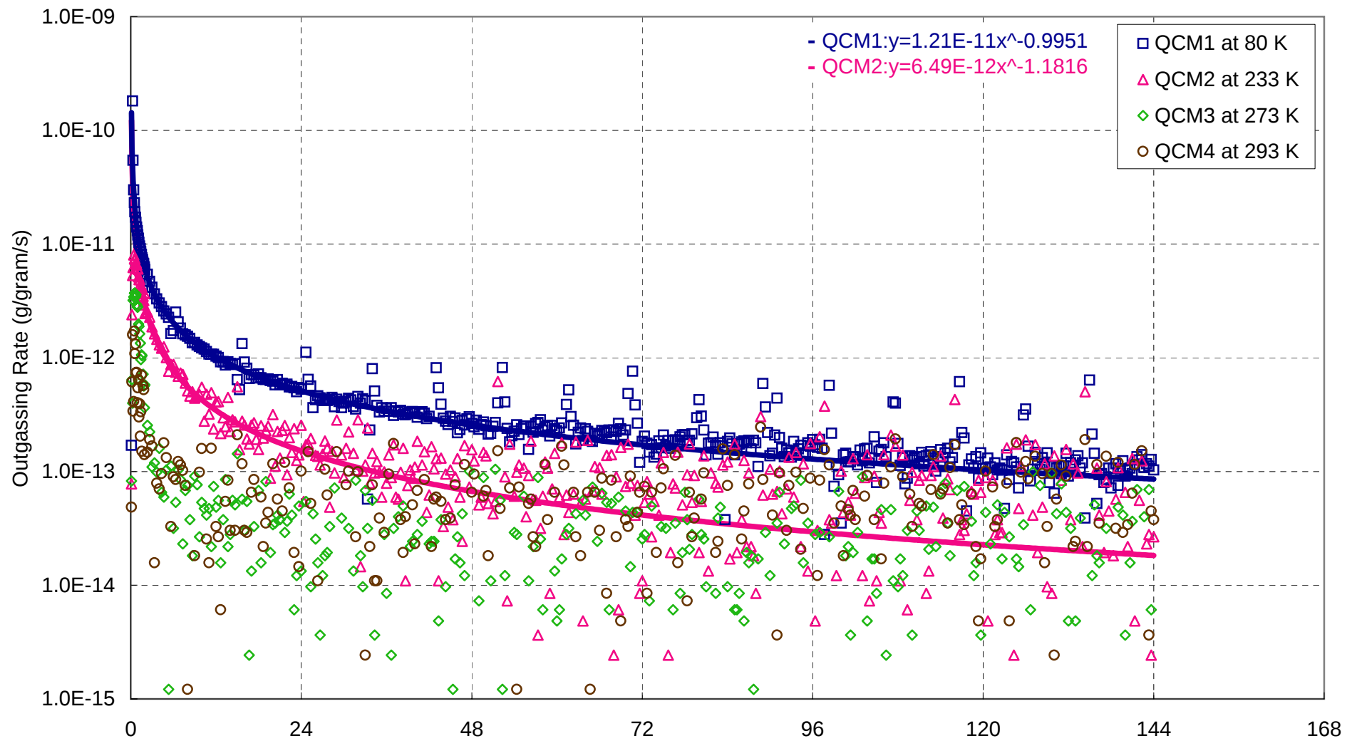
Fig.3 Outgassing Rate from Sample as a Function of Time during the Isothermal Outgassing Test on Nonwoven Fabric (H8004) at 60
