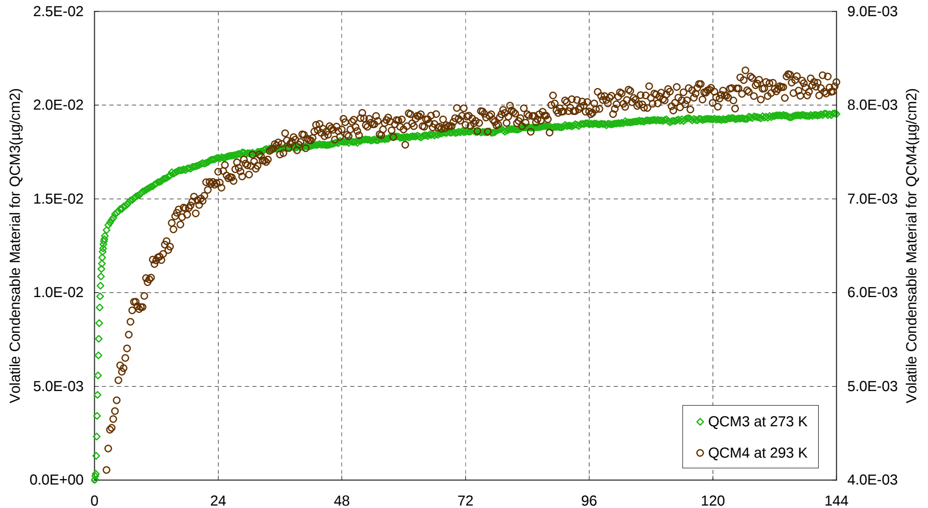
Fig.2 Volatile Condensable Material for QCMs at 0 and 20 as a Function of Time during the Isothermal Outgassing Test on Nonwoven Fabric (H8004) at 60
