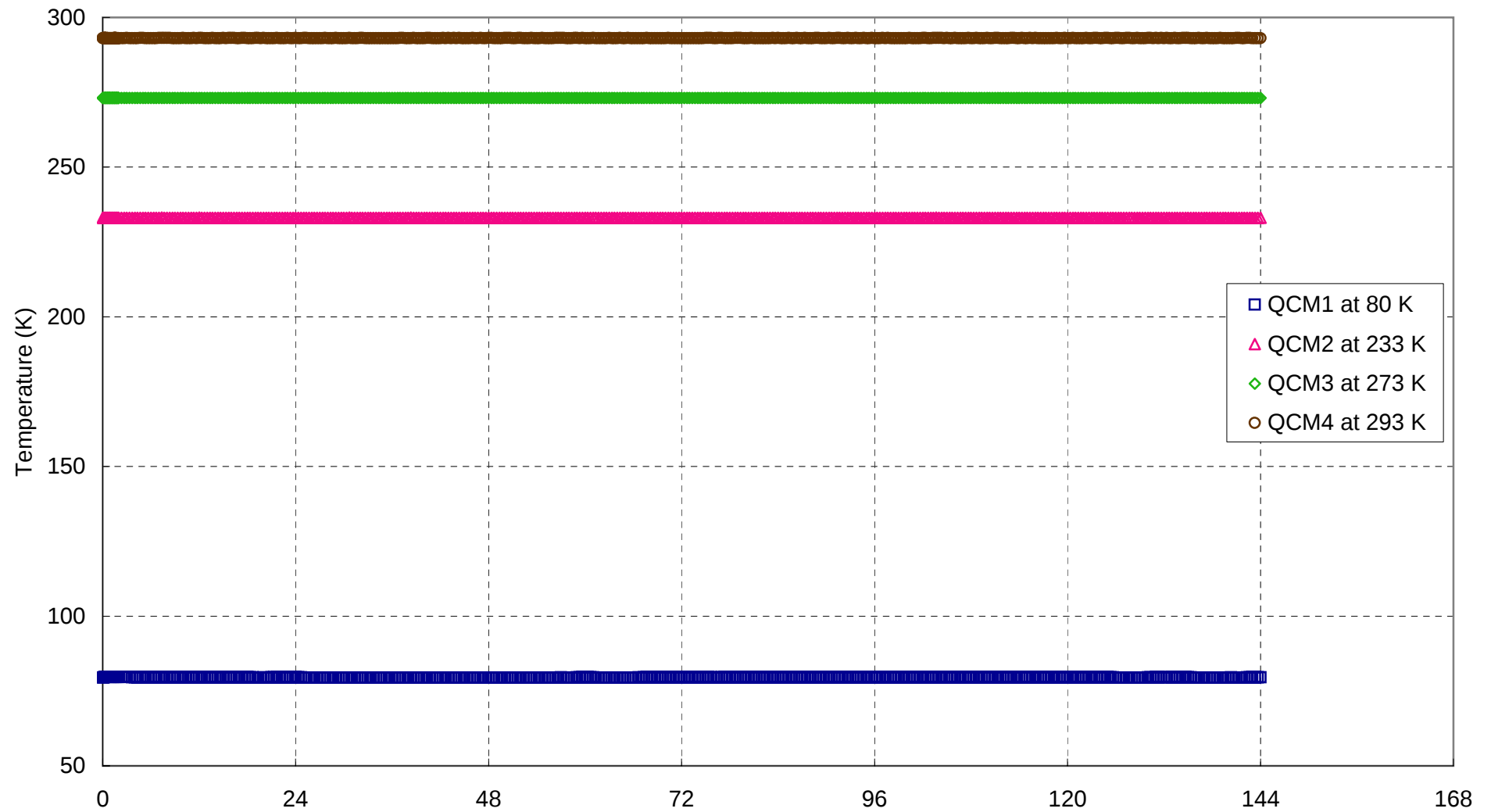
Fig.4 Temperature as a Function of Time during the Isothermal Outgassing Test on Nonwoven Fabric (H8004) at 60
