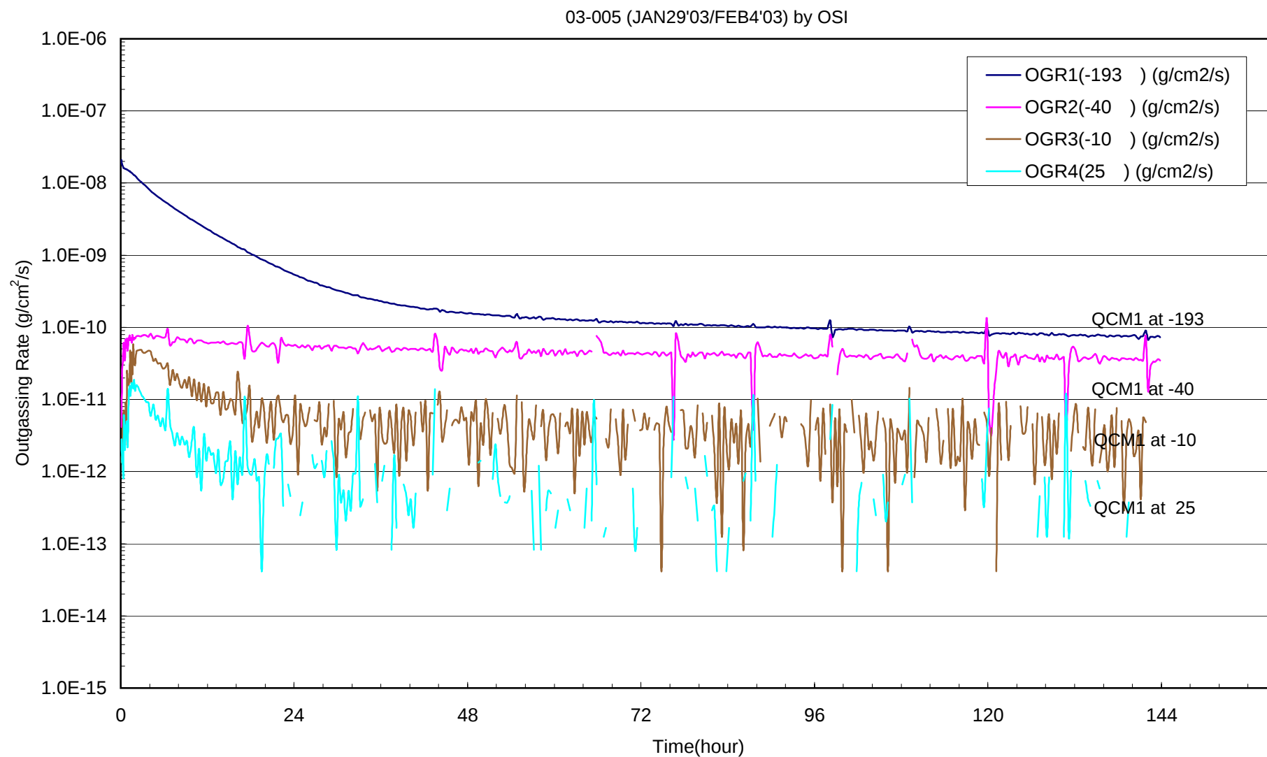
Fig.2 Outgassing Rate from Sample as a Function of Time during the Isothermal Outgassing Test on Solithane 113/C113-300 at 79.3 .
