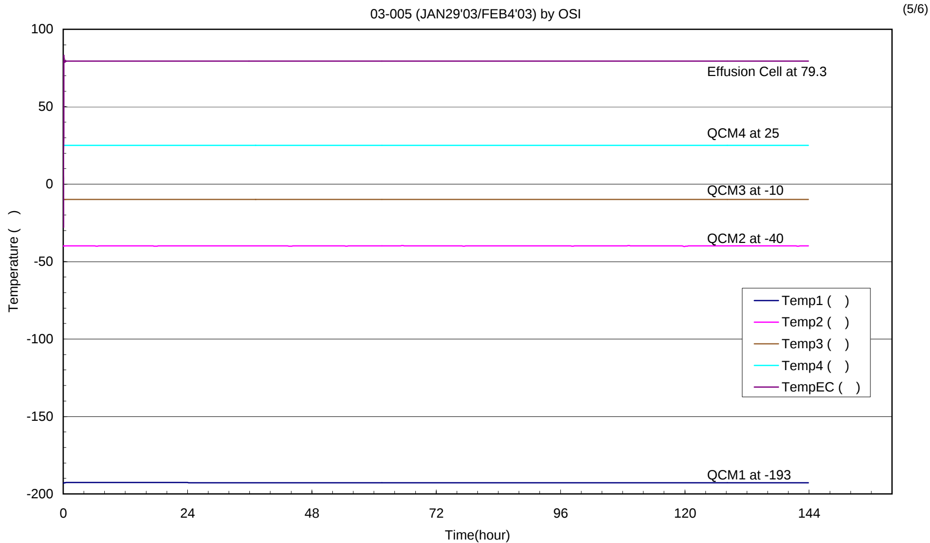
Fig.3 Temperature Fluctuation as a Function of Time during the Isothermal Outgassing Test on Solithane 113/C113-300 at 79.3 °C .
