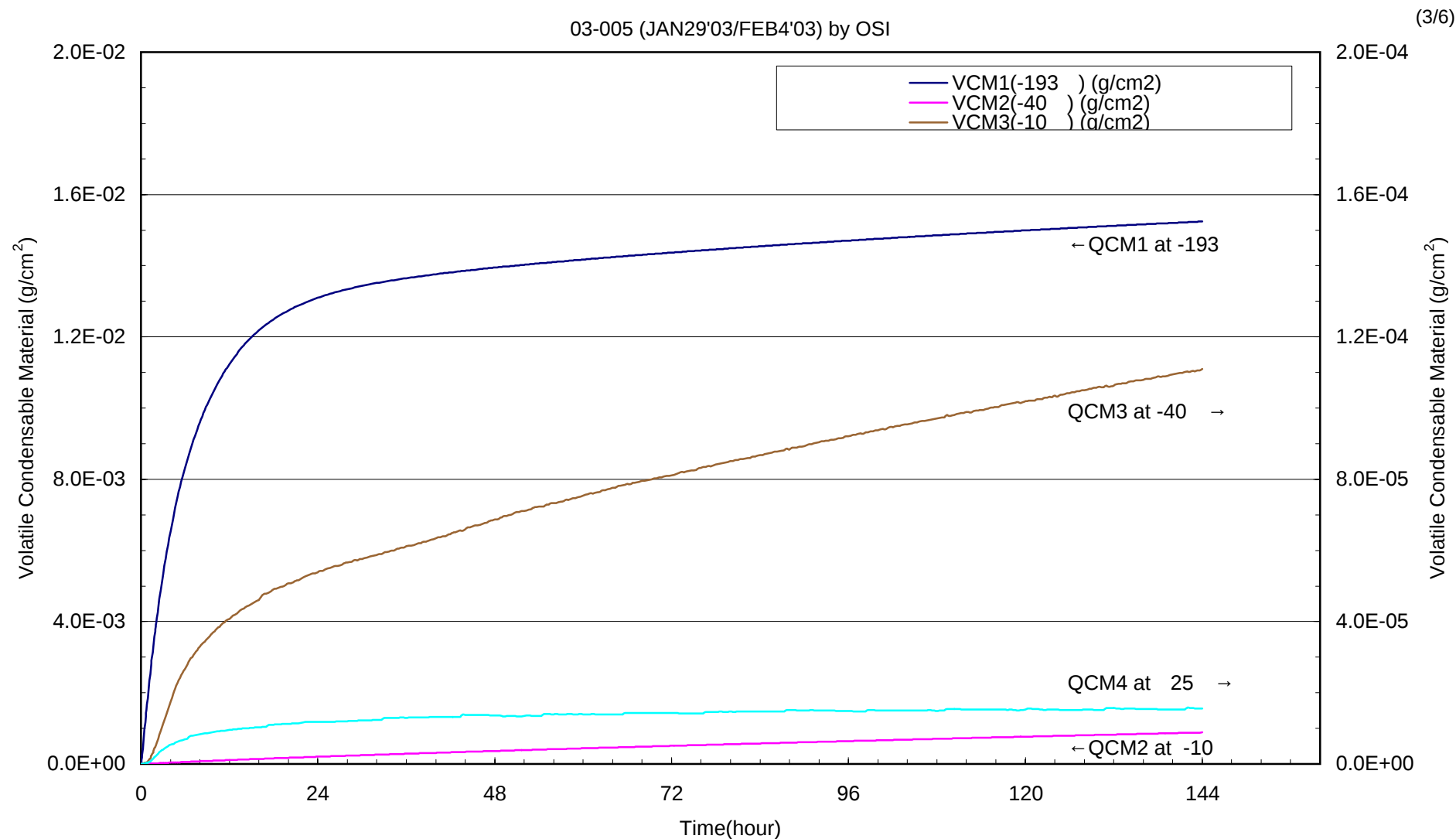
Fig.1 Volatile Condensable Material for QCMs at -193 , -40 , -10 and 25 as a Function of Time during the Isothermal Outgassing Test on Solithane 113/C113-300 at 79.3 .
