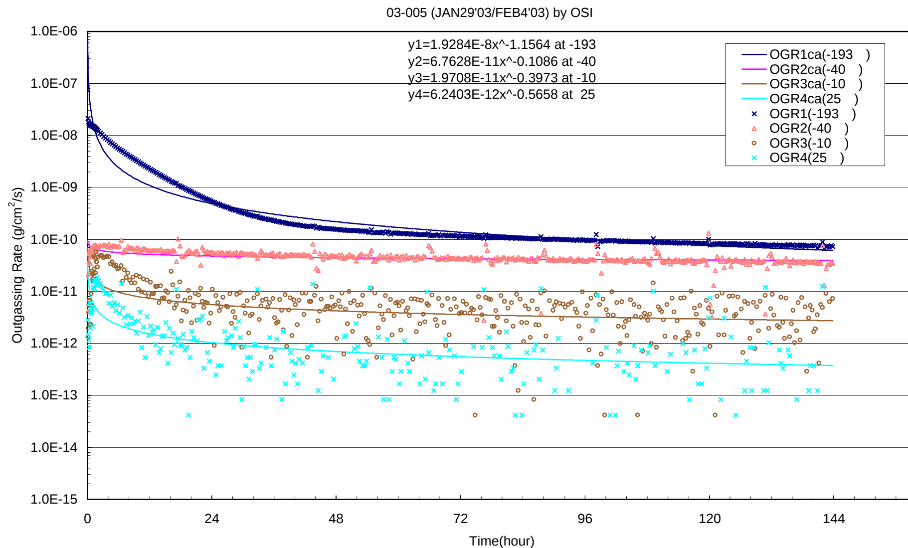
Fig.4 Outgassing Rate from Sample as a Function of Time during the Isothermal Outgassing Test on Solithane 113/C113-300 at 79.3 (with Fitting Curves).
