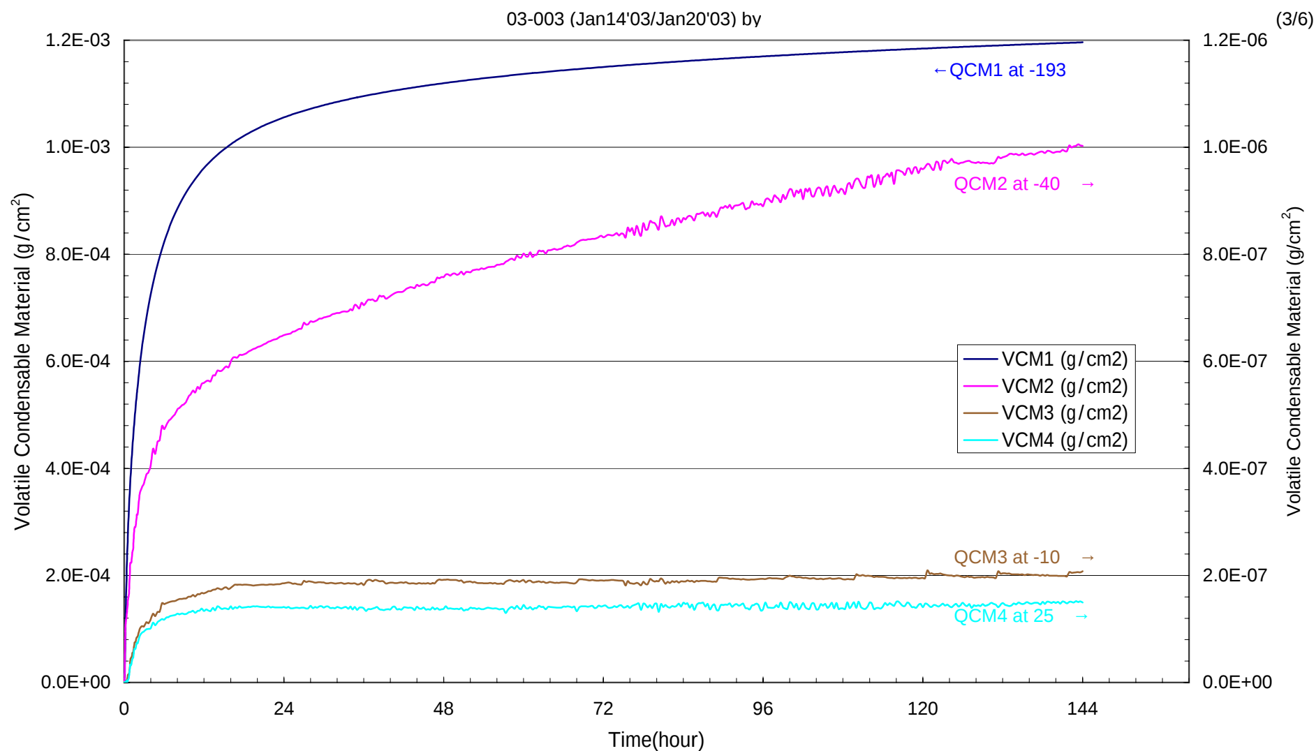
Fig.1 Volatile Condensable Material for QCMs at -193 , -40 , -10 and 25 as a Function of Time during the Isothermal Outgassing Test on Aeroglaze Black Paint at 46.0 .
