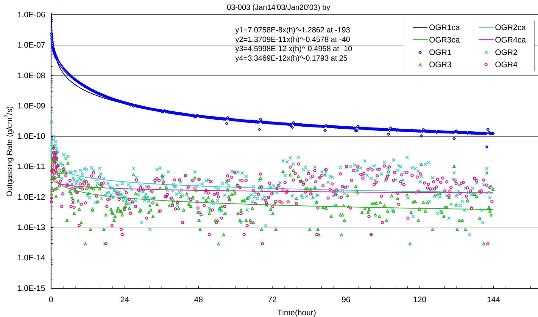
Fig.4 Outgassing Rate from Sample as a Function of Time during the Isothermal Outgassing Test on Aeroglaze Black Paint at 46.0 (with Fitting Curves).
