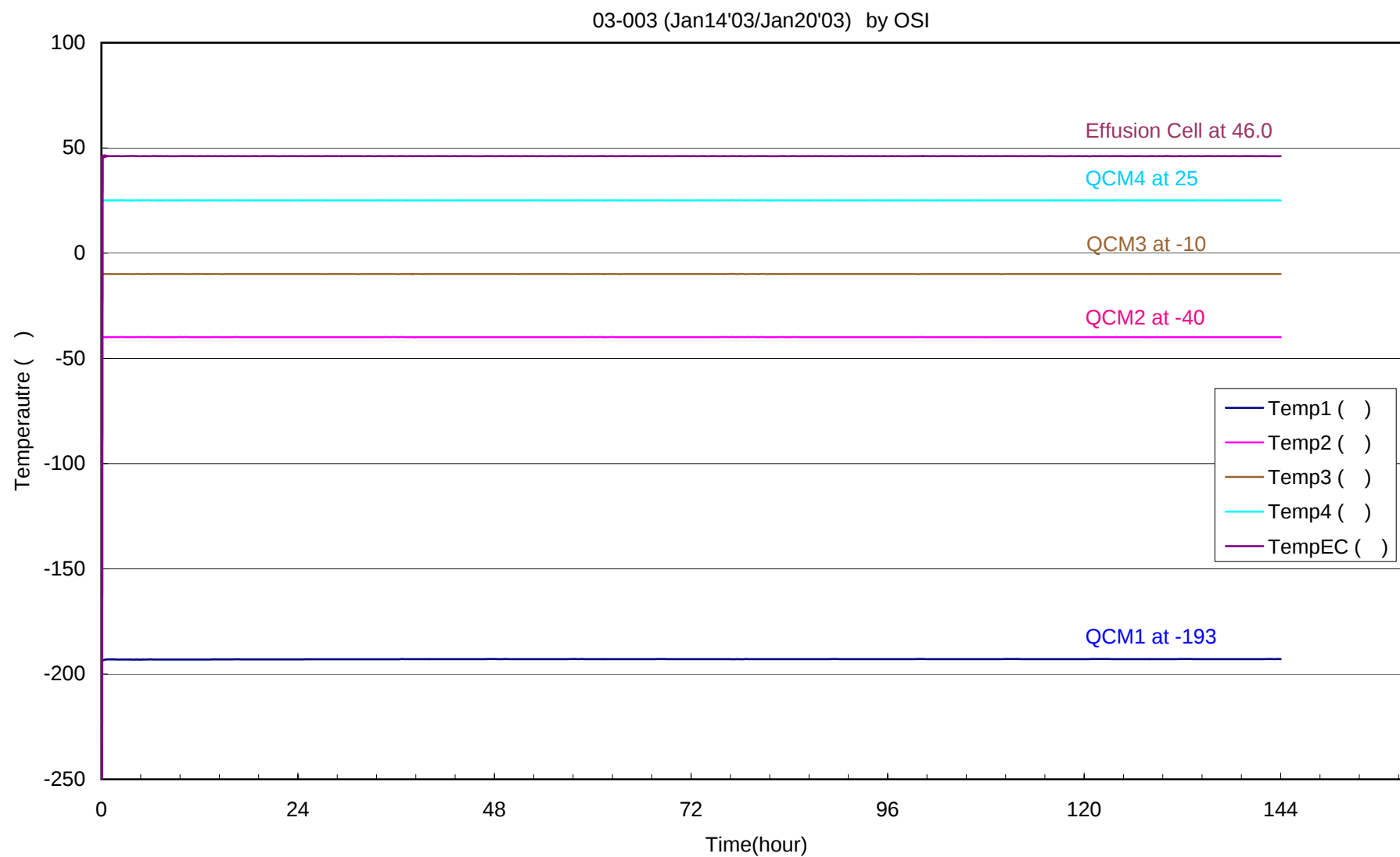
Fig.3 Temperature Fluctuation as a Function of Time during the Isothermal Outgassing Test on Aeroglaze Black Paint at 46.0 °C .
