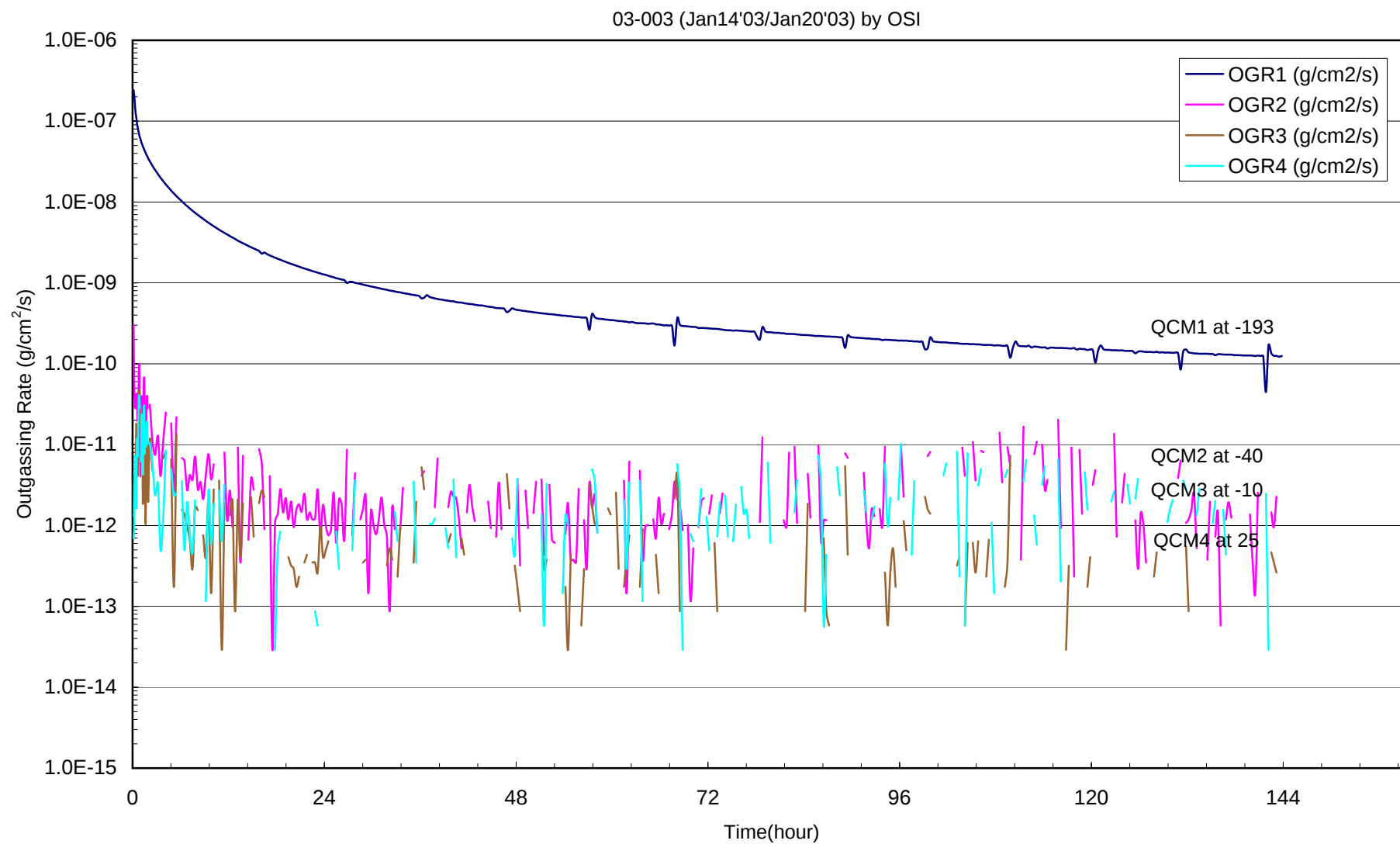
Fig.2 Outgassing Rate from Sample as a Function of Time during the Isothermal Outgassing Test on Aeroglaze Black Paint at 46.0 °C.
