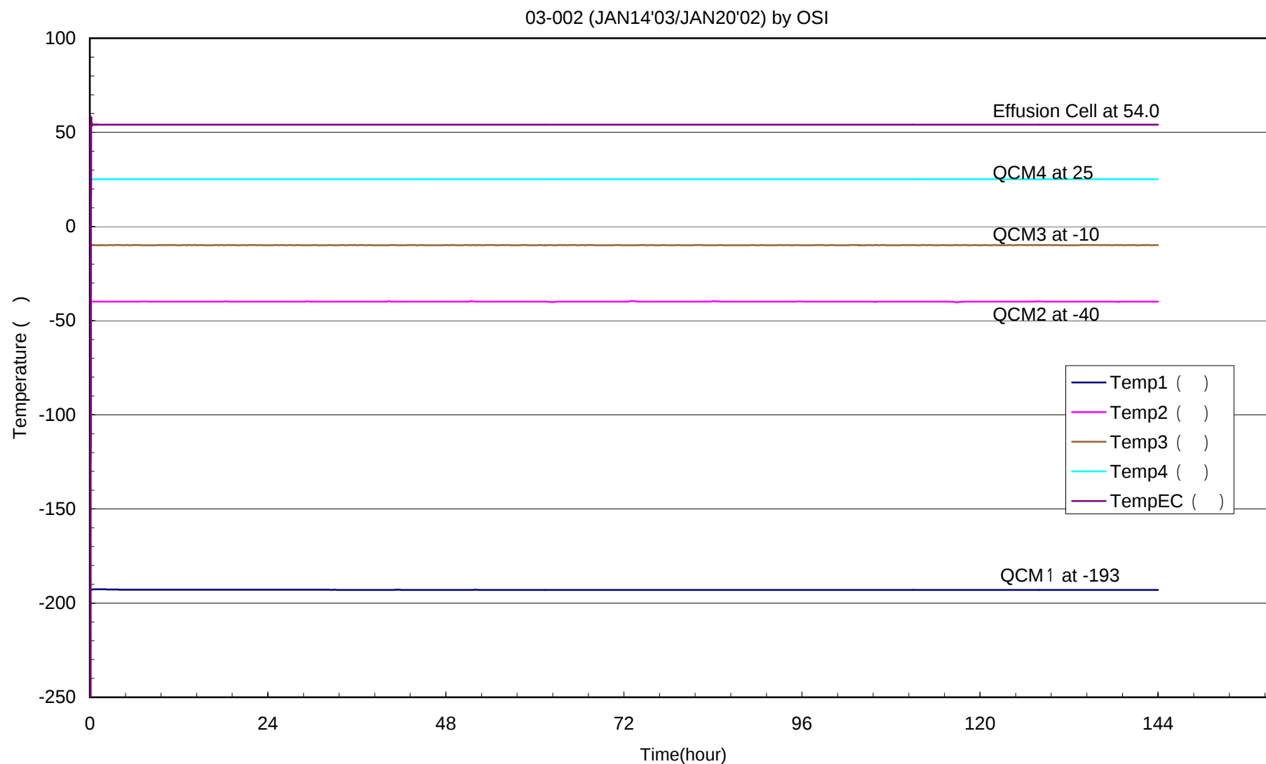
Fig.3 Temperature Fluctuation as a Function of Time during the Isothermal Outgassing Test on Cable NASDA-QTS-1064 at 54.0 .
