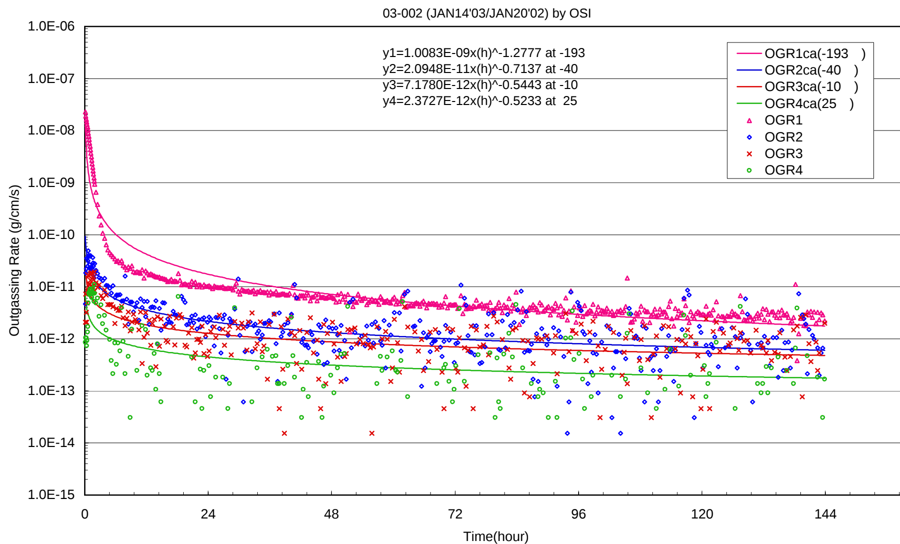
Fig.4 Outgassing Rate from Sample as a Function of Time during the Isothermal Outgassing Test on Cable NASDA-QTS-1064 at 54 (with Fitting curves).
