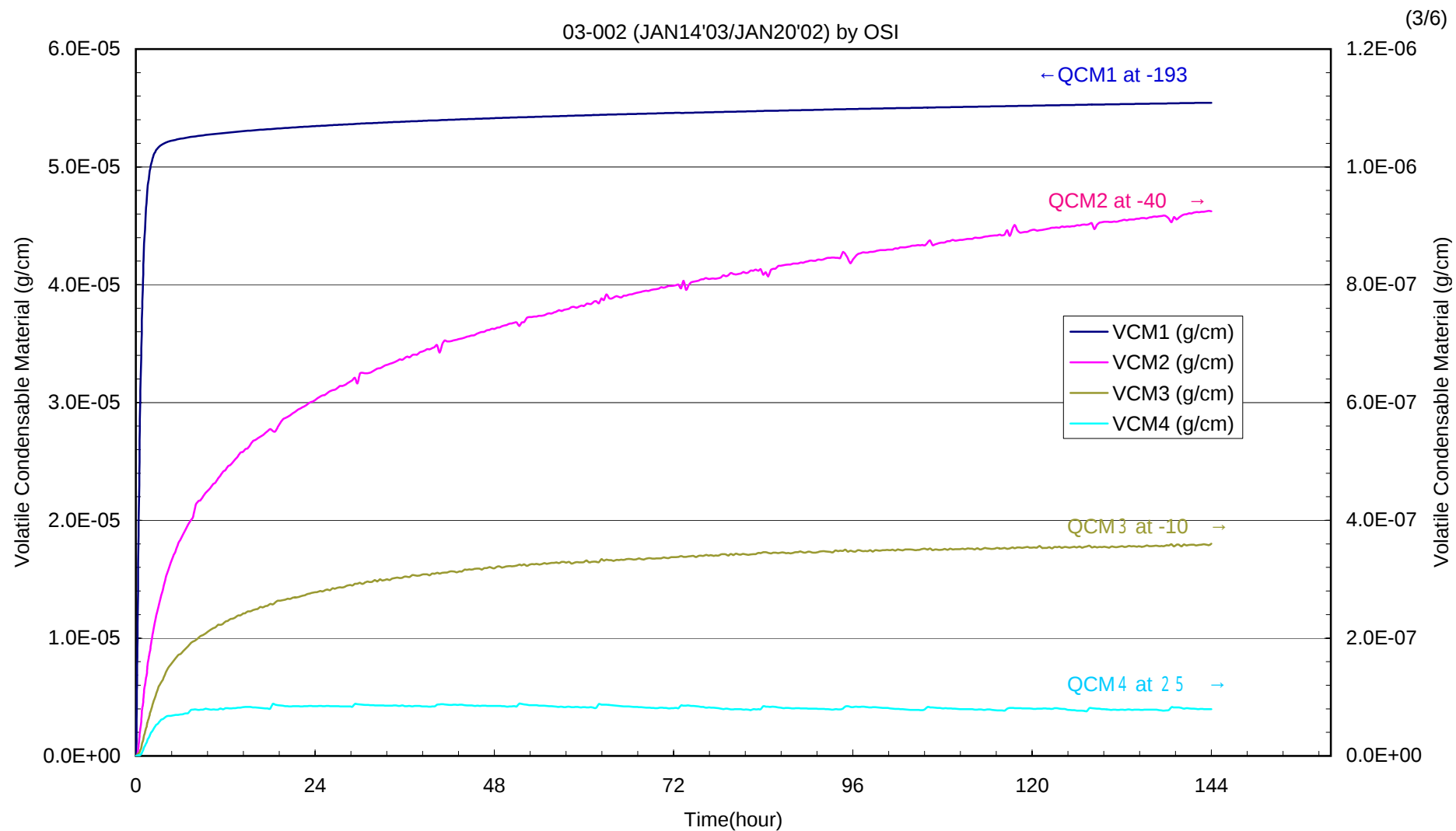
Fig.1 Volatile Condensable Material for QCMs at -193 , -40 , -10 and 25 as a Function of Time during the Isothermal Outgassing Test on Cable NASDA-QTS-1064 at 54 .
