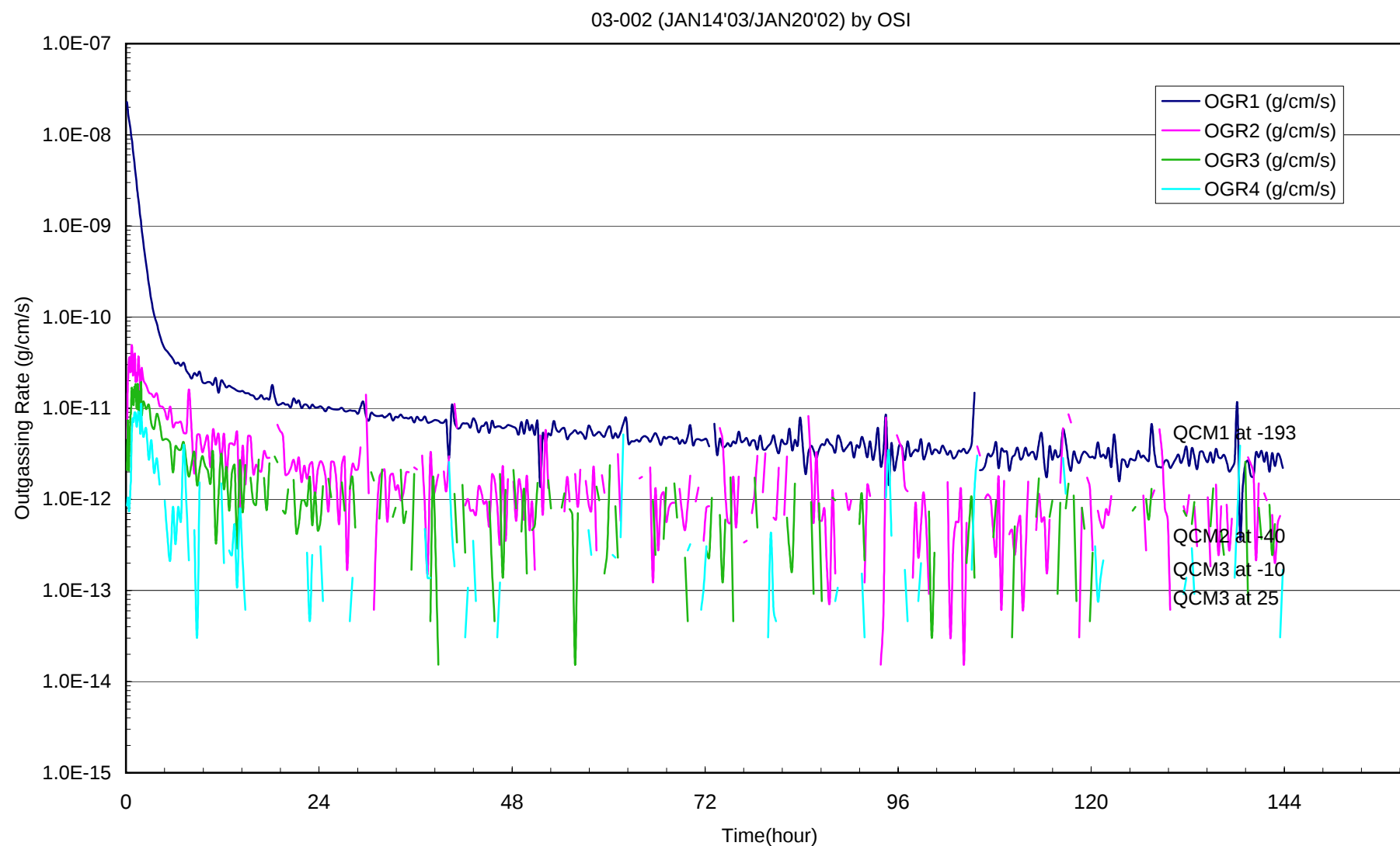
Fig.2 Outgassing Rate from Sample as a Function of Time during the Isothermal Outgassing Test on Cable NASDA-QTS-1064 at 54 .
