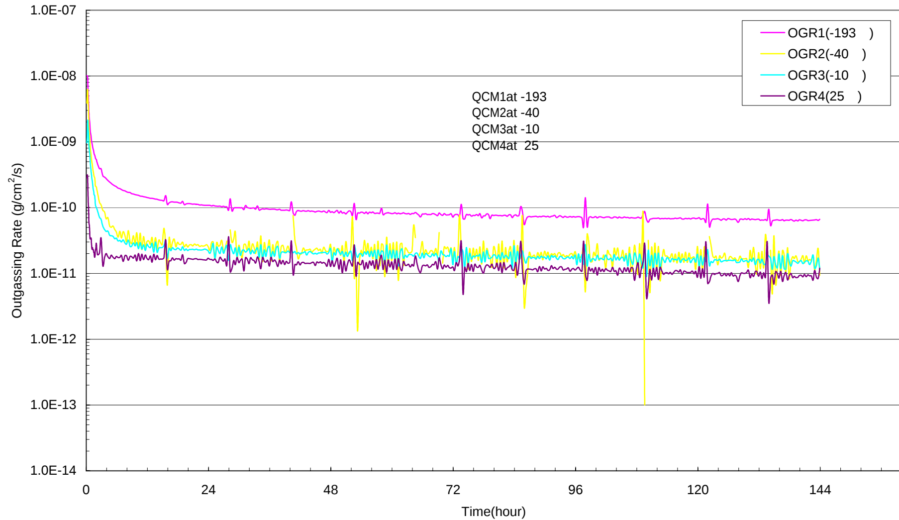
Fig.2 Outgassing Rate from Sample as a Function of Time during the Isothermal Outgassing Test on Scotch 79 Tape at 125 °C (Raw Data only).
