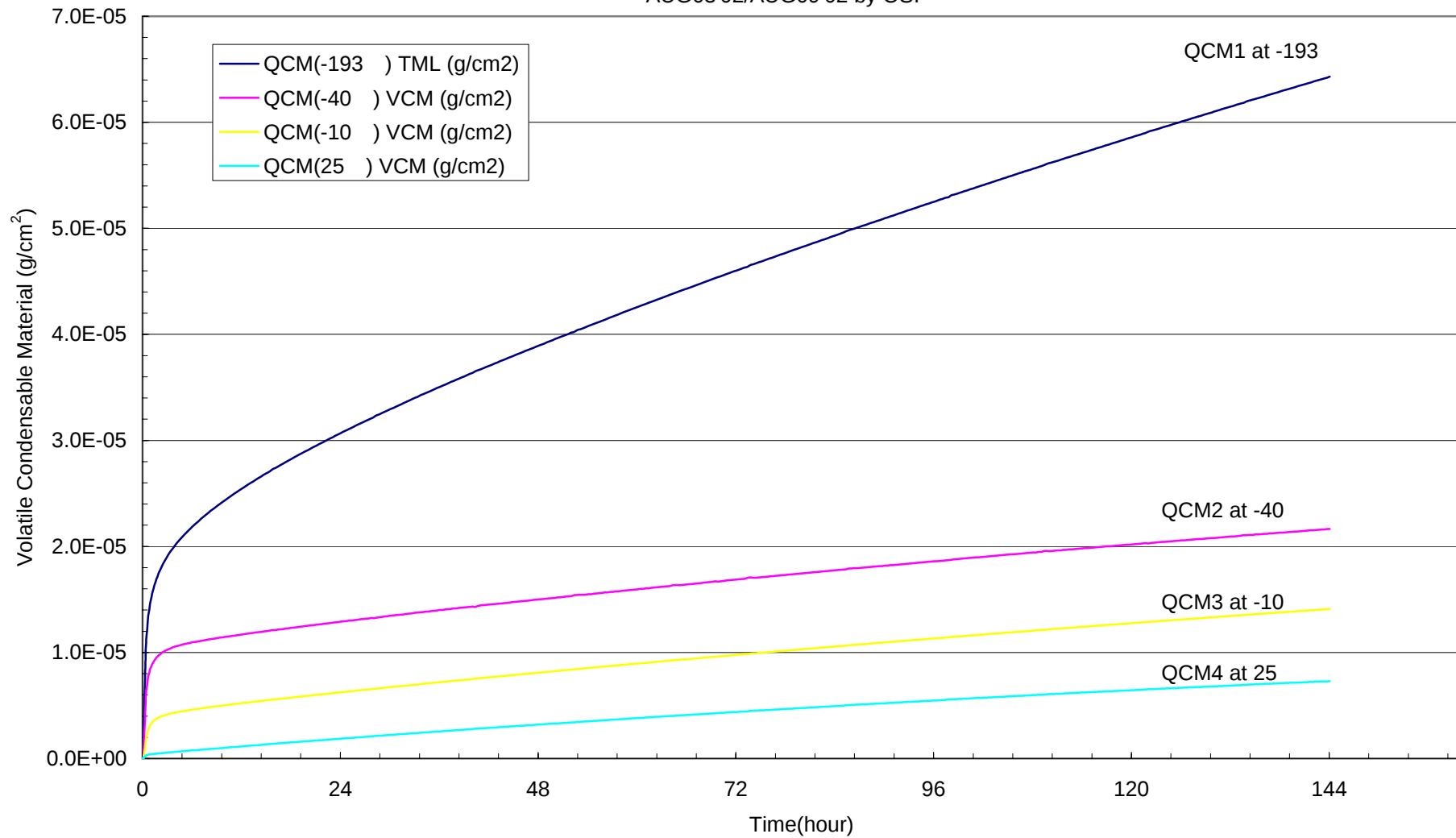
Fig.1 Volatile Condensable Material for QCMs at -193 , -40 , -10 and 25 as a Function of Time during the Isothermal Outgassing Test on Scotch 79 Tape at 125 .
