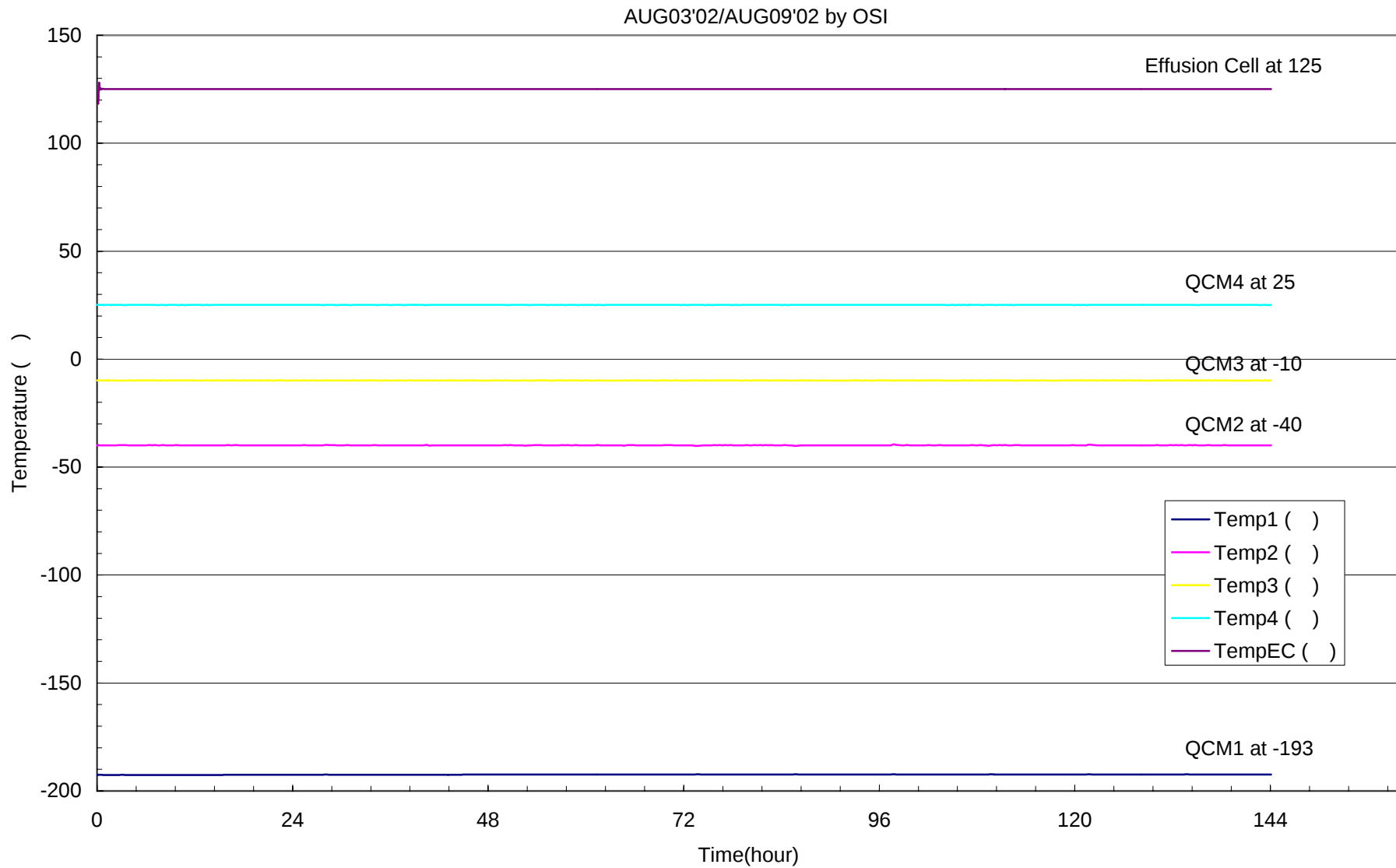
Fig.3 Temperature Fluctuation as a Function of Time during the Isothermal Outgassing Test on Scotch 79 Tape at 125 °C .
